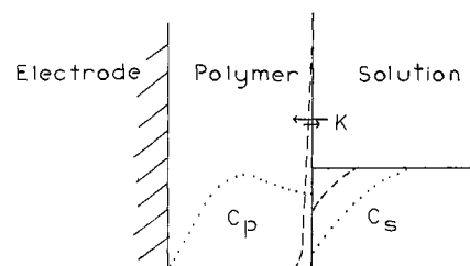
Figure 6. Schematic concentration profiles during permeation chromatographic experiment. (—) Initial profile at t = 0 ; (---) profile after electrode immersion in solution at relatively short times; (···) profile at longer time.
